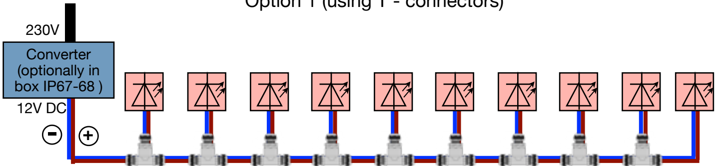
Option 1 (using T - connectors)
